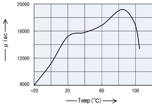
\mu_{iac} vs. Temperature \mu_{iac} 温度特性
