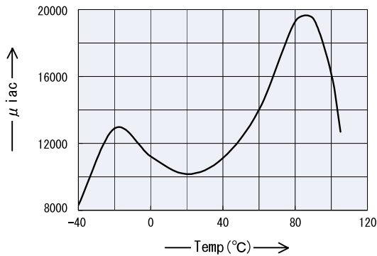
\mu_{iac} vs. Temperature \mu_{iac} 温度特性
