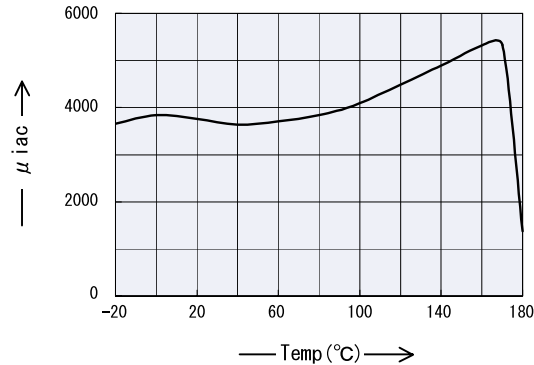
\mu_{iac} vs. Temperature \mu_{iac} 温度特性
