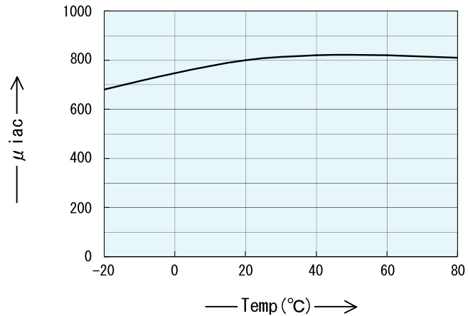
\mu_{iac} vs. Temperature \mu_{iac} 温度特性
