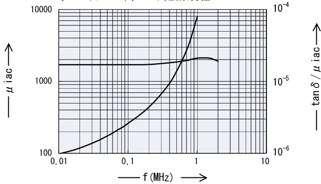
\mu_{iac} and \tan \delta / \mu_{iac} vs. Frequency \mu_{iac} 及 \tan \delta / \mu_{iac} 周波数特性
