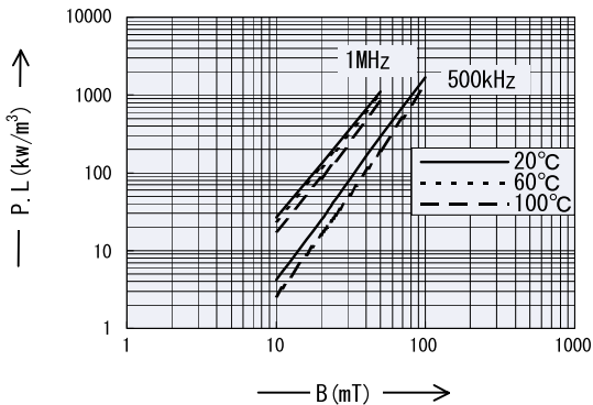
Power loss vs. Flux density P \cdot L vs. 磁束密度
