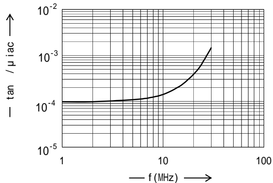
\tan / \mu_{iac} vs. Frequency \tan / \mu_{iac} 周波数特性
